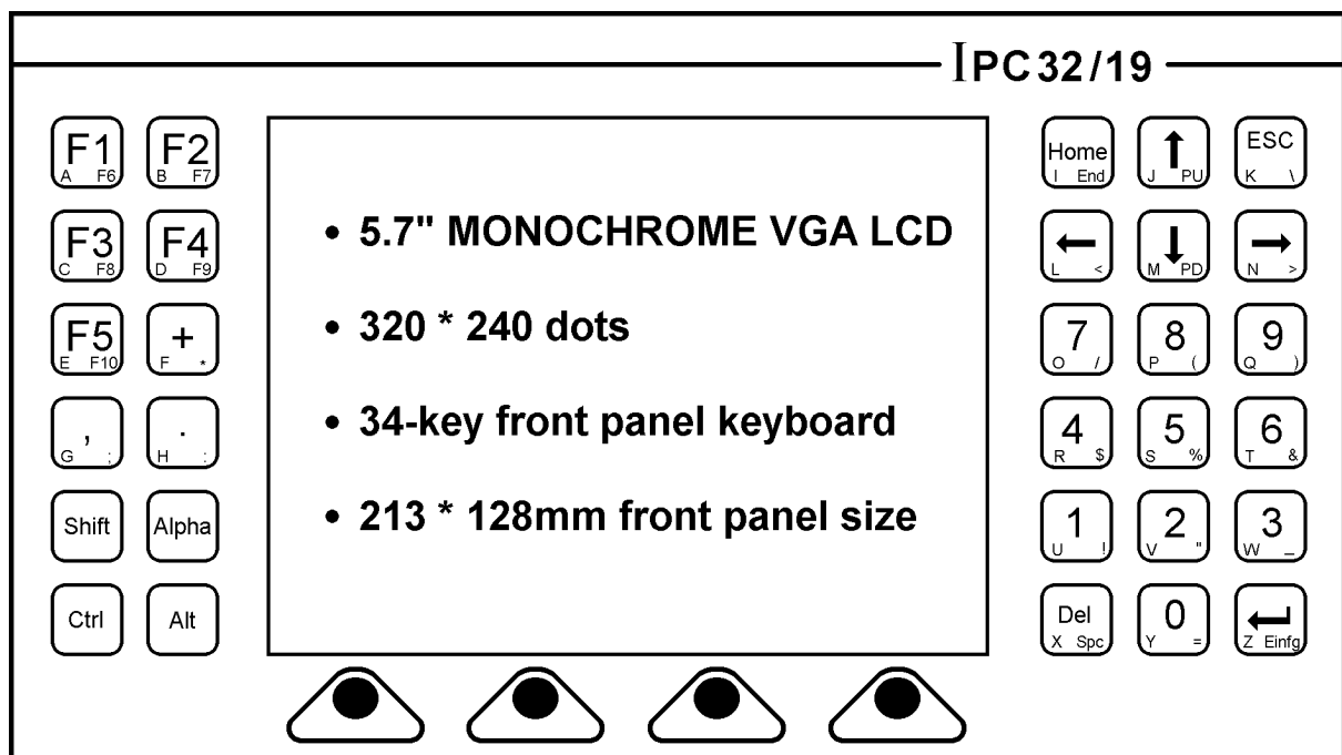
Figure 1: IPC32/19 Front Panel Keyboard
