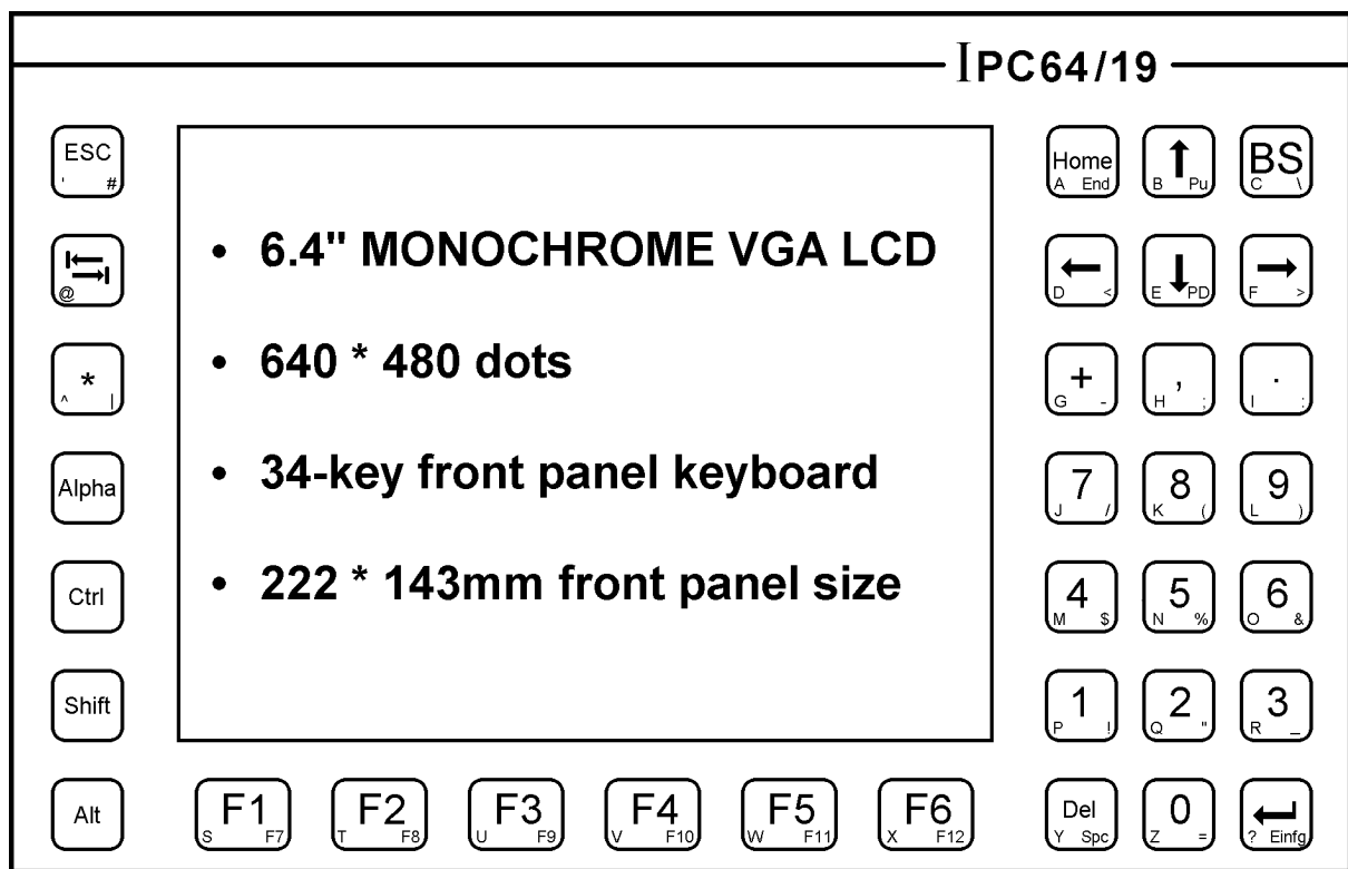
Figure 1: IPC64/19M Front Panel Keyboard
