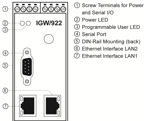
Basic hardware interfaces of the IGW/922
