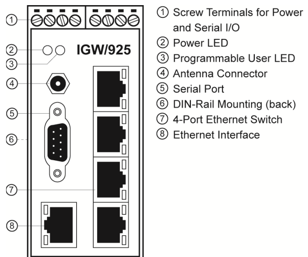
Basic hardware interfaces of the IGW/925-U
