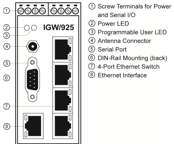
Basic hardware interfaces of the IGW/925-W
