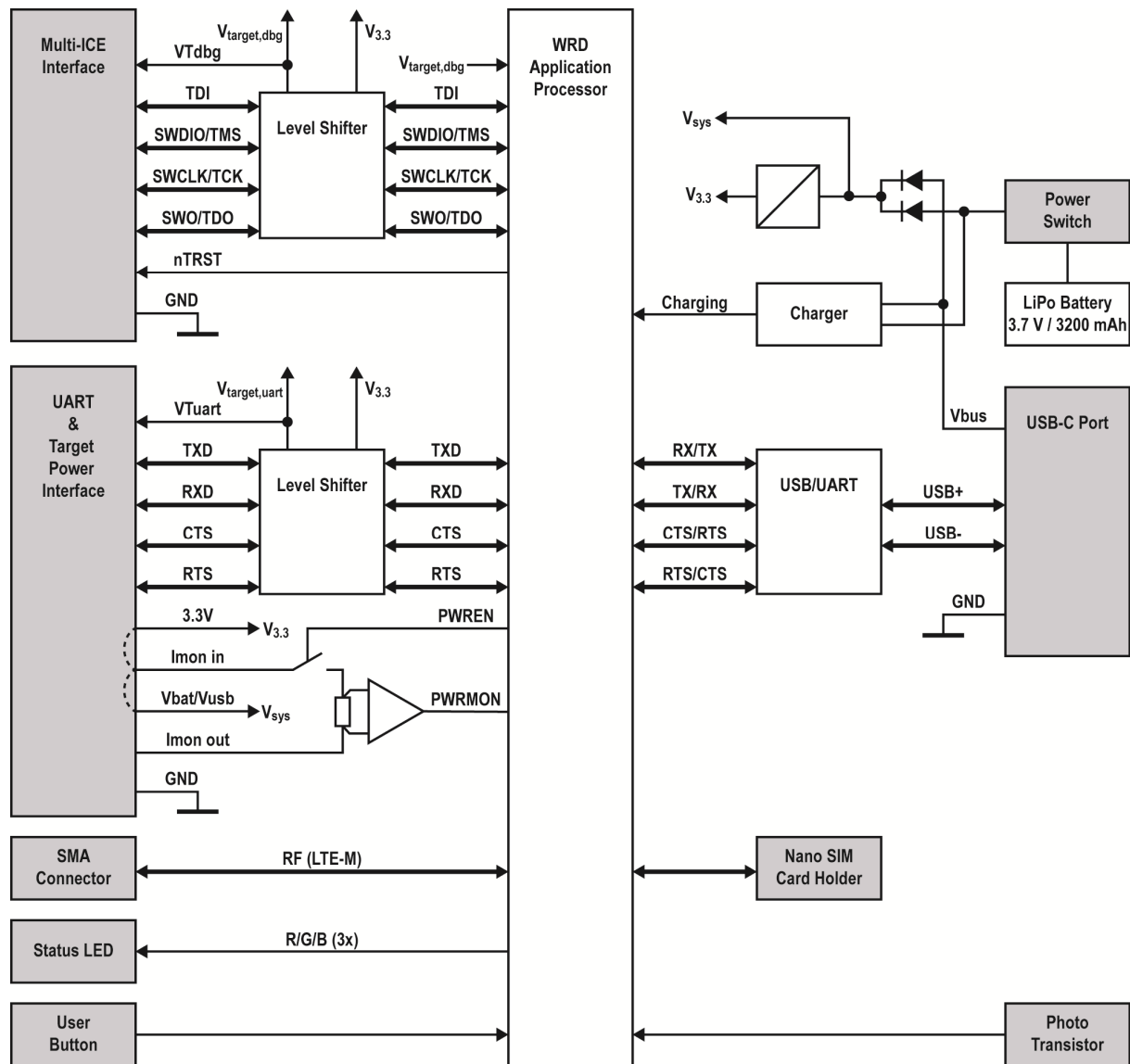
Figure 2: Block diagram of WRD/Probe
