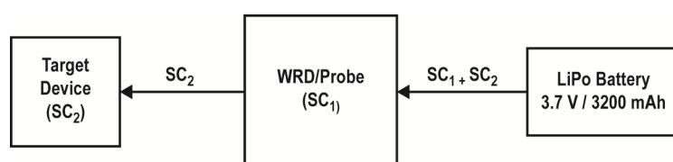
Figure 7: Composition of the total power consumption of the WRD/Probe
